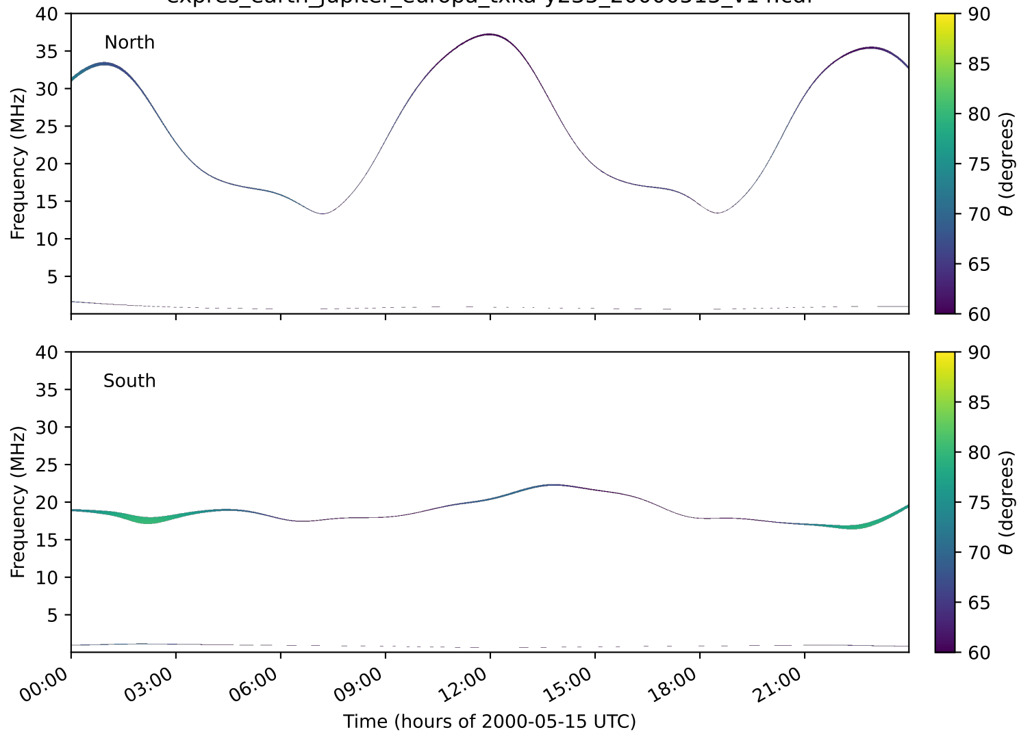
expres_earth_jupiter_europa_txka-y235_20000515_v14.cdf
