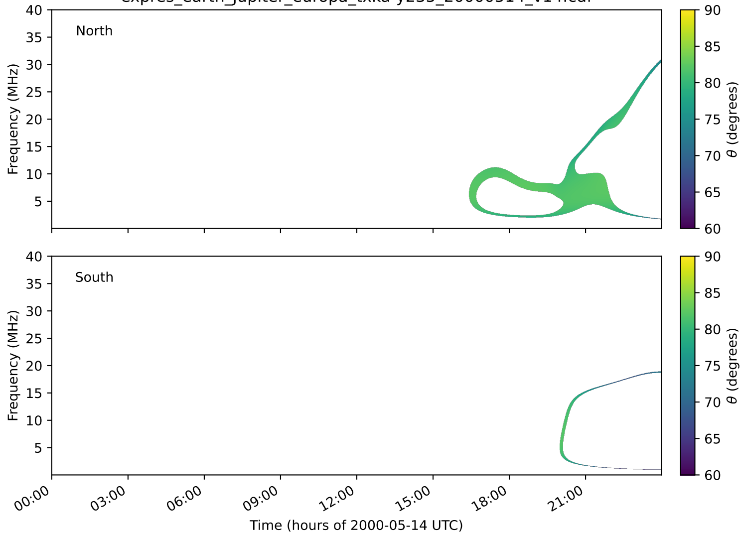
expres_earth_jupiter_europa_txka-y235_20000514_v14.cdf
