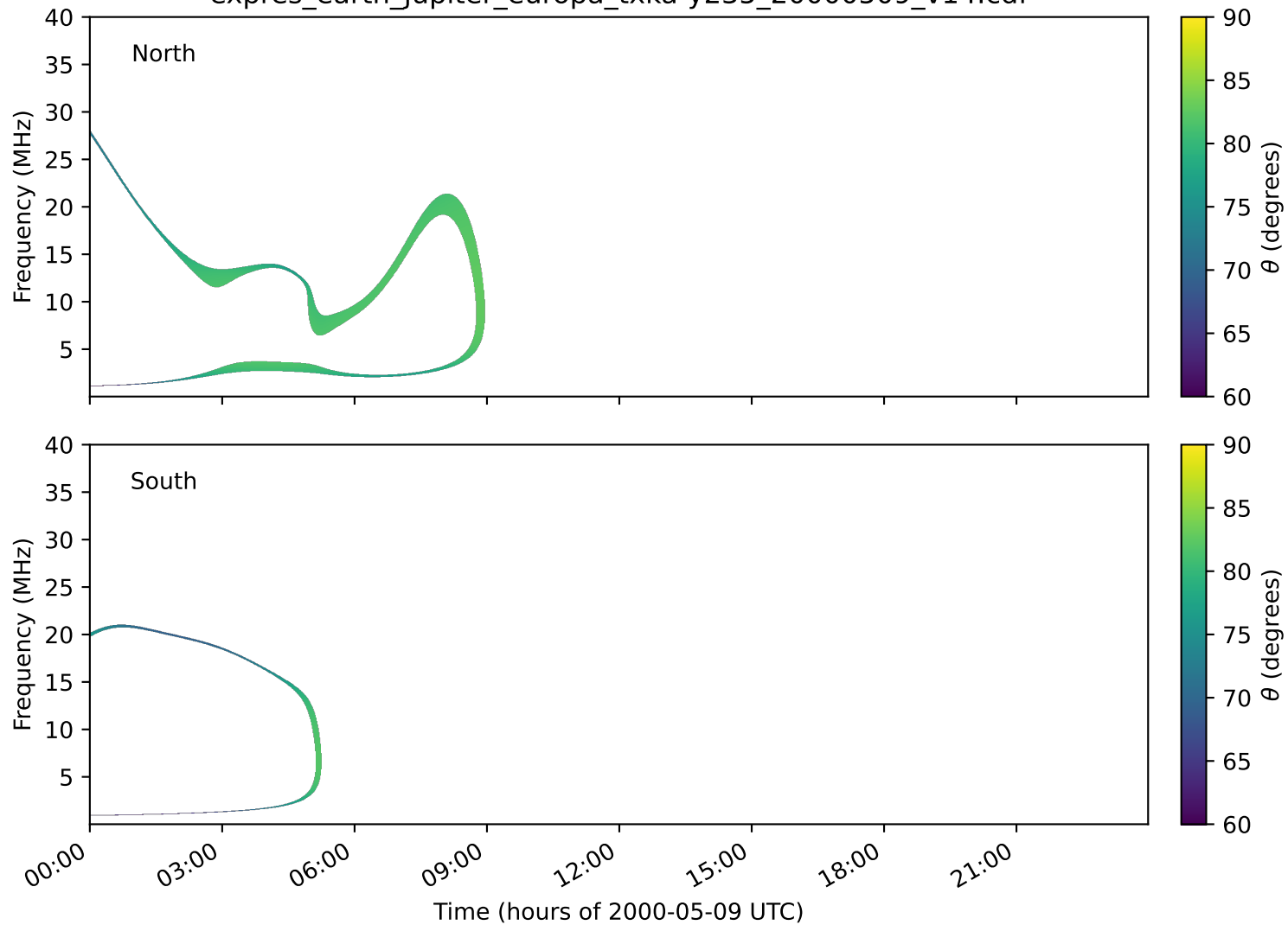
expres_earth_jupiter_europa_txka-y235_20000509_v14.cdf
