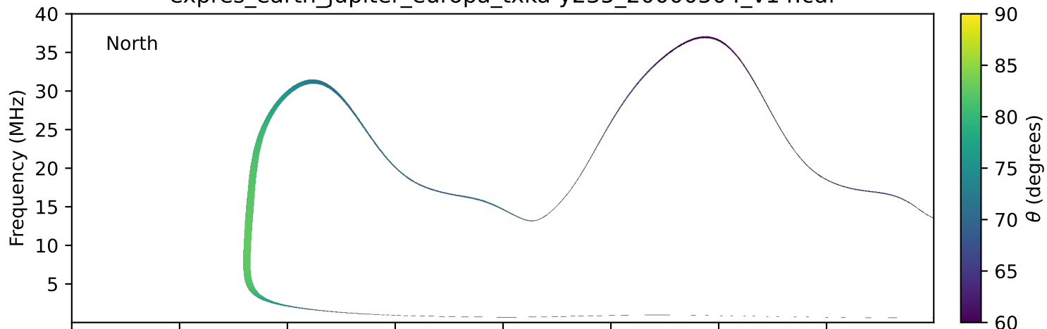
expres_earth_jupiter_europa_txka-y235_20000504_v14.cdf
