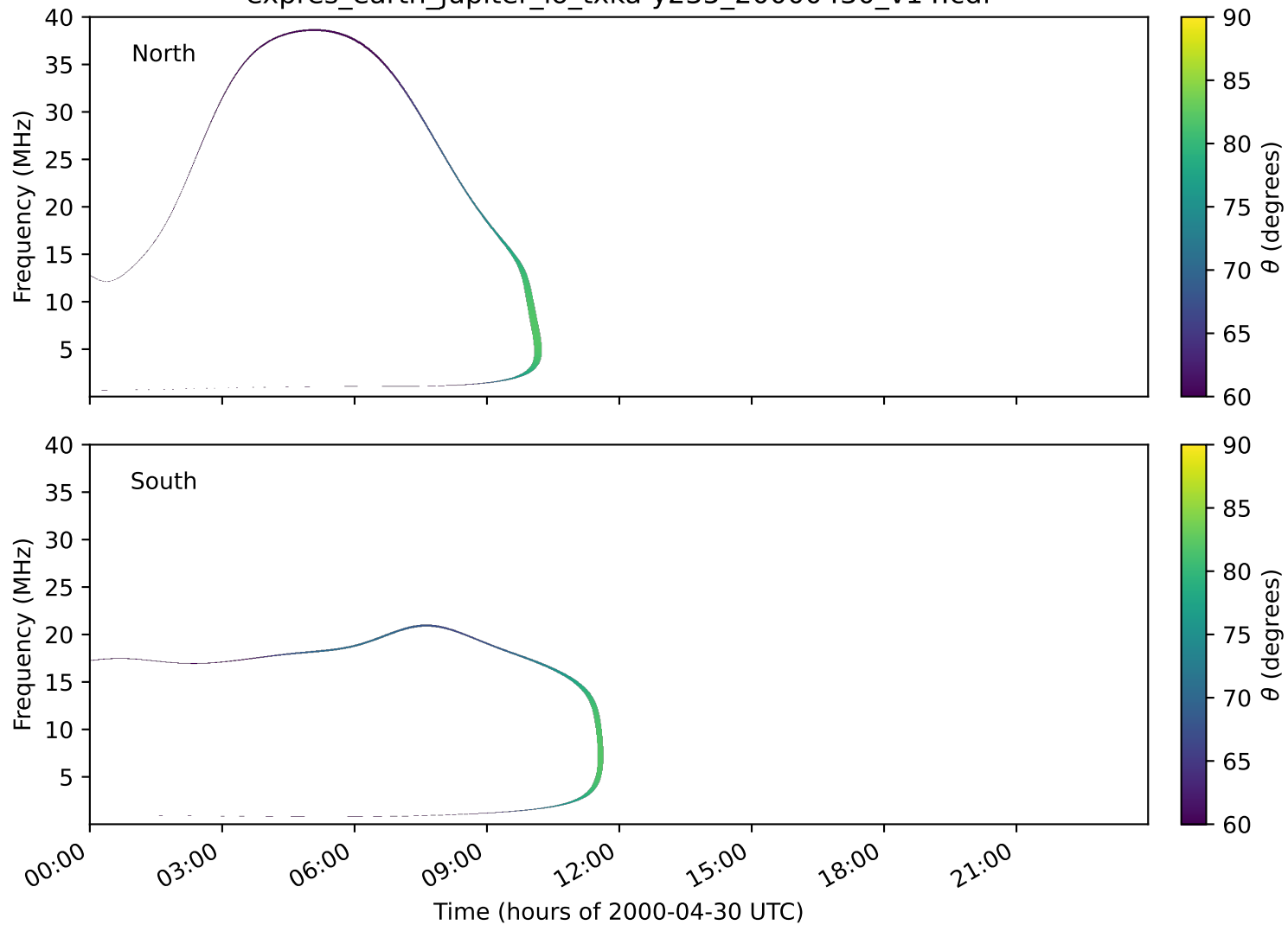
expres_earth_jupiter_io_txka-y235_20000430_v14.cdf
