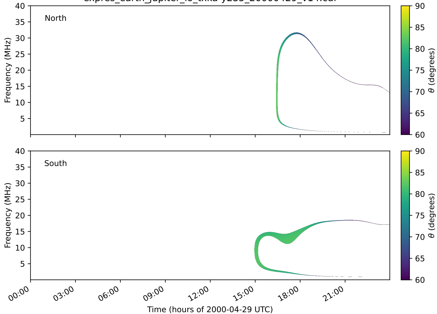
expres_earth_jupiter_io_txka-y235_20000429_v14.cdf
