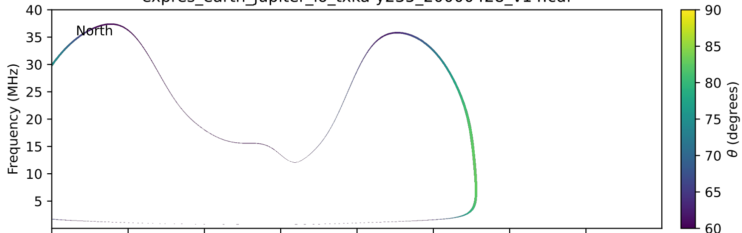
expres_earth_jupiter_io_txka-y235_20000428_v14.cdf
