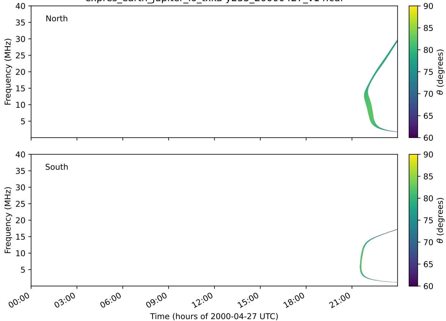
expres_earth_jupiter_io_txka-y235_20000427_v14.cdf
