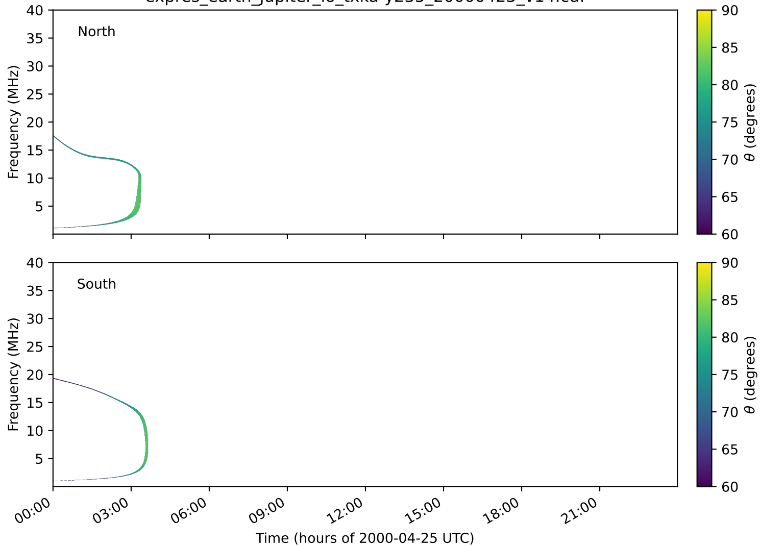
expres_earth_jupiter_io_txka-y235_20000425_v14.cdf
