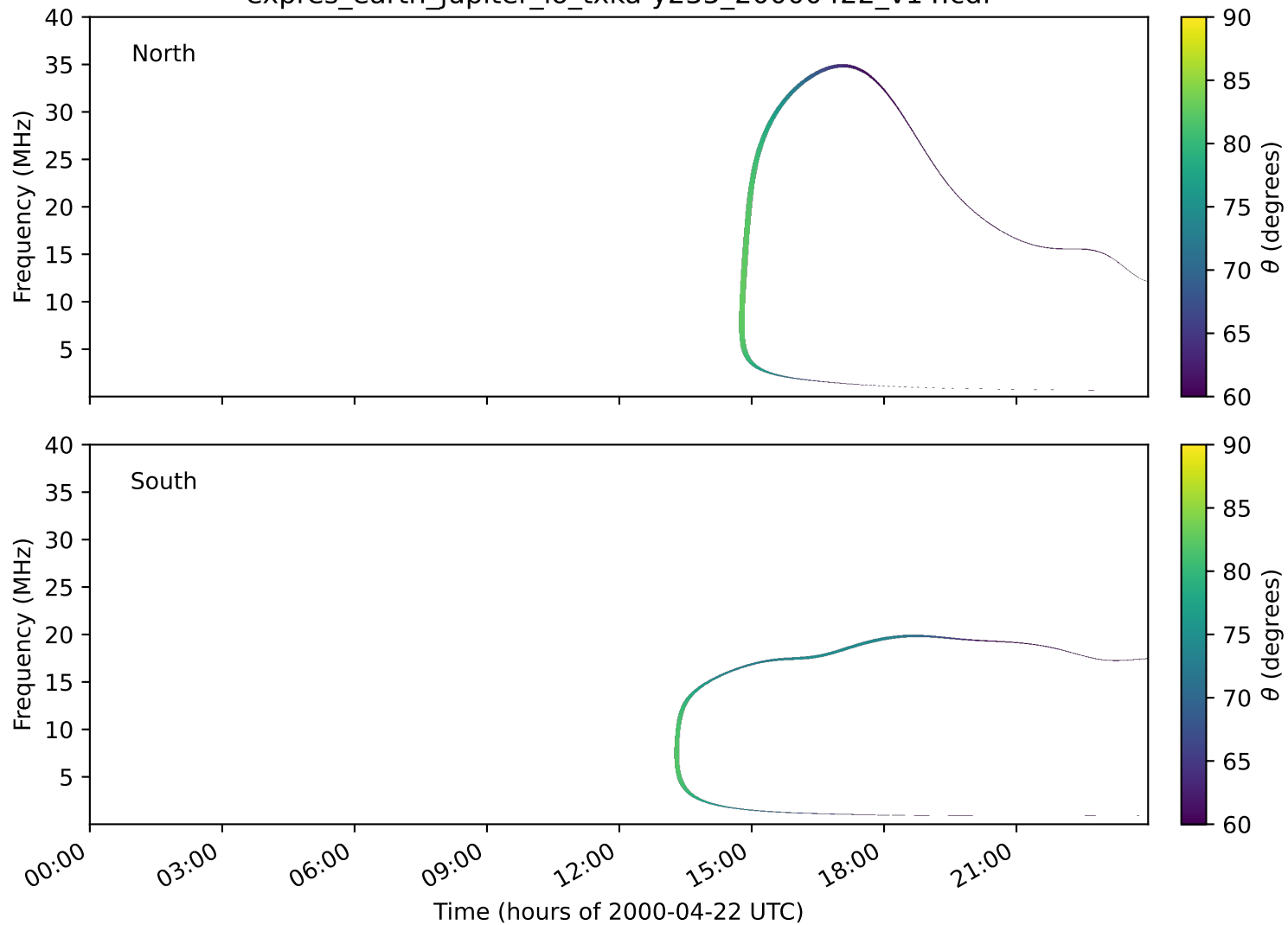
expres_earth_jupiter_io_txka-y235_20000422_v14.cdf
