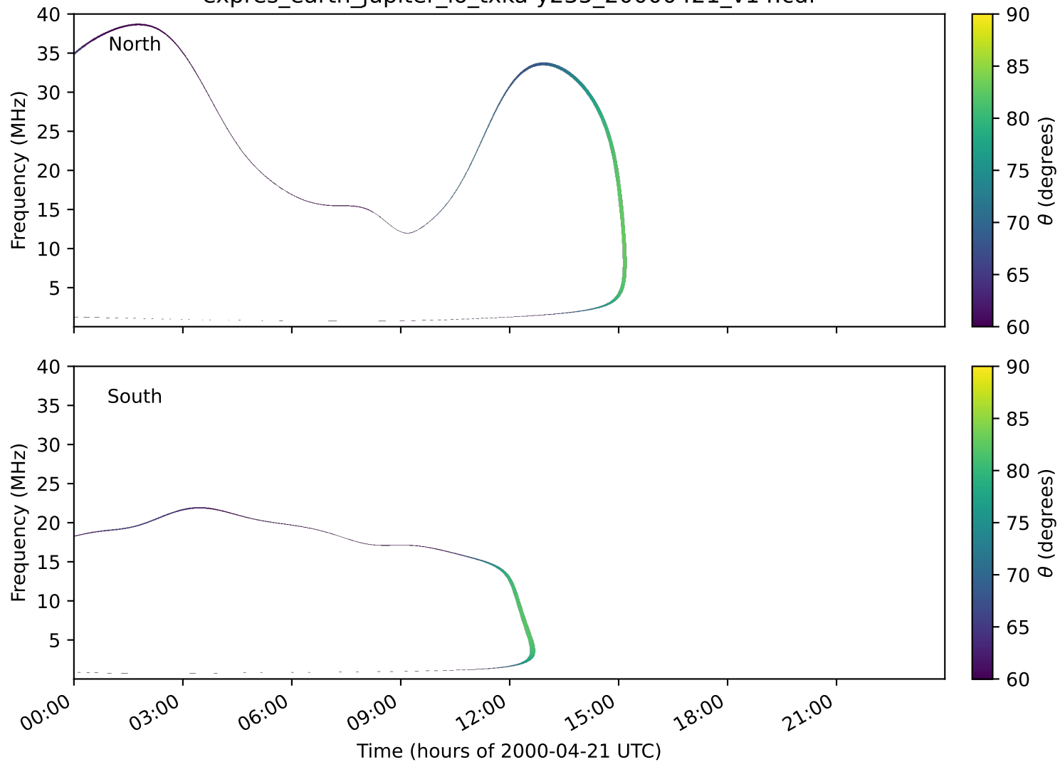
expres_earth_jupiter_io_txka-y235_20000421_v14.cdf
