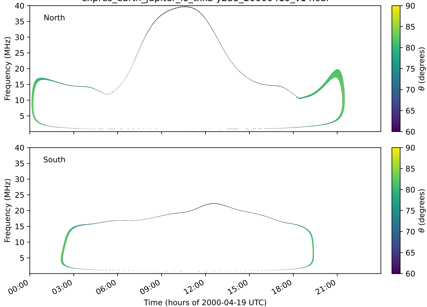
expres_earth_jupiter_io_txka-y235_20000419_v14.cdf
