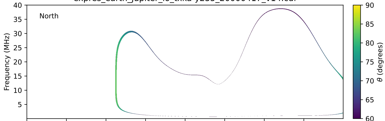
expres_earth_jupiter_io_txka-y235_20000417_v14.cdf
