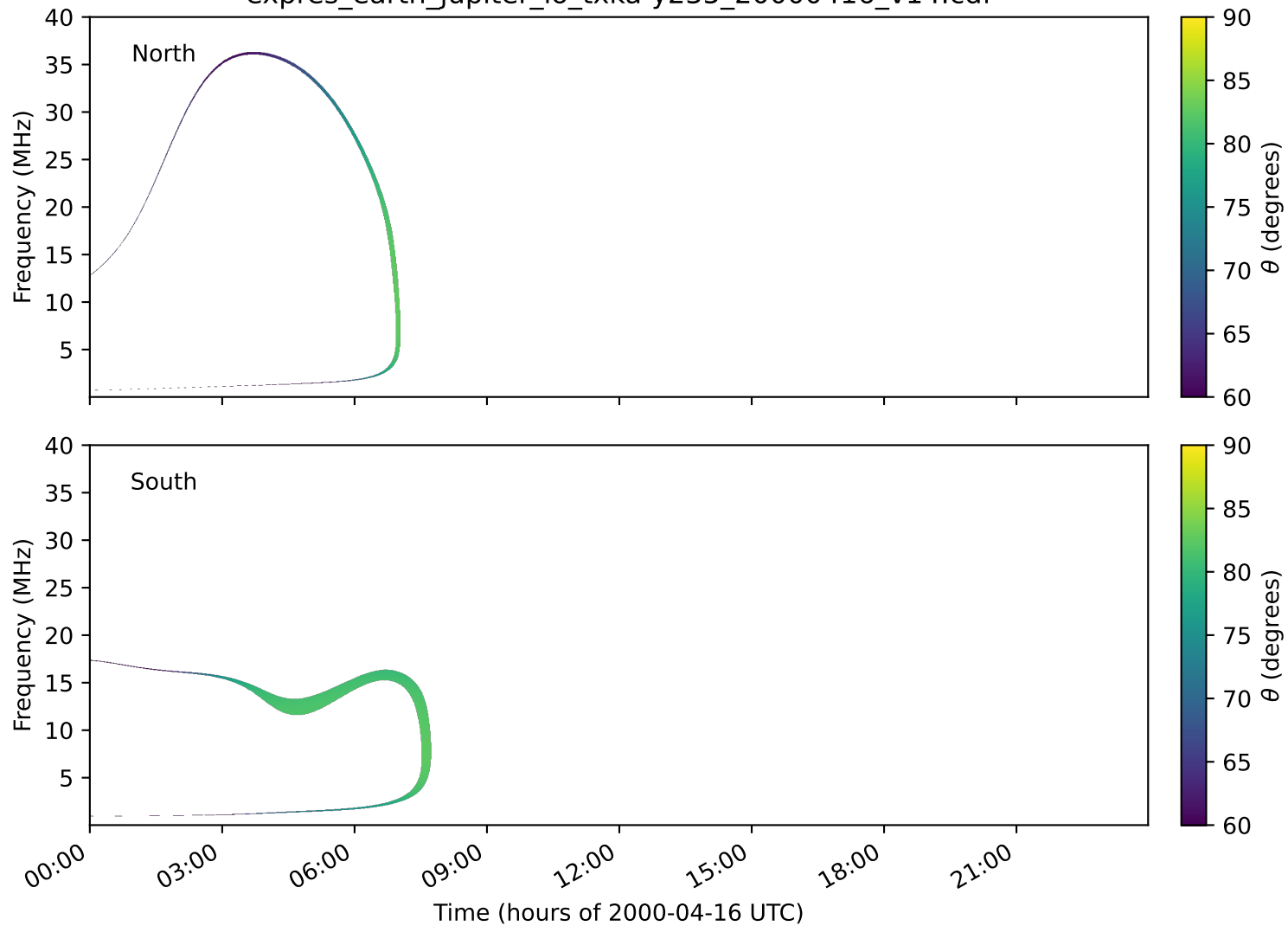
expres_earth_jupiter_io_txka-y235_20000416_v14.cdf
