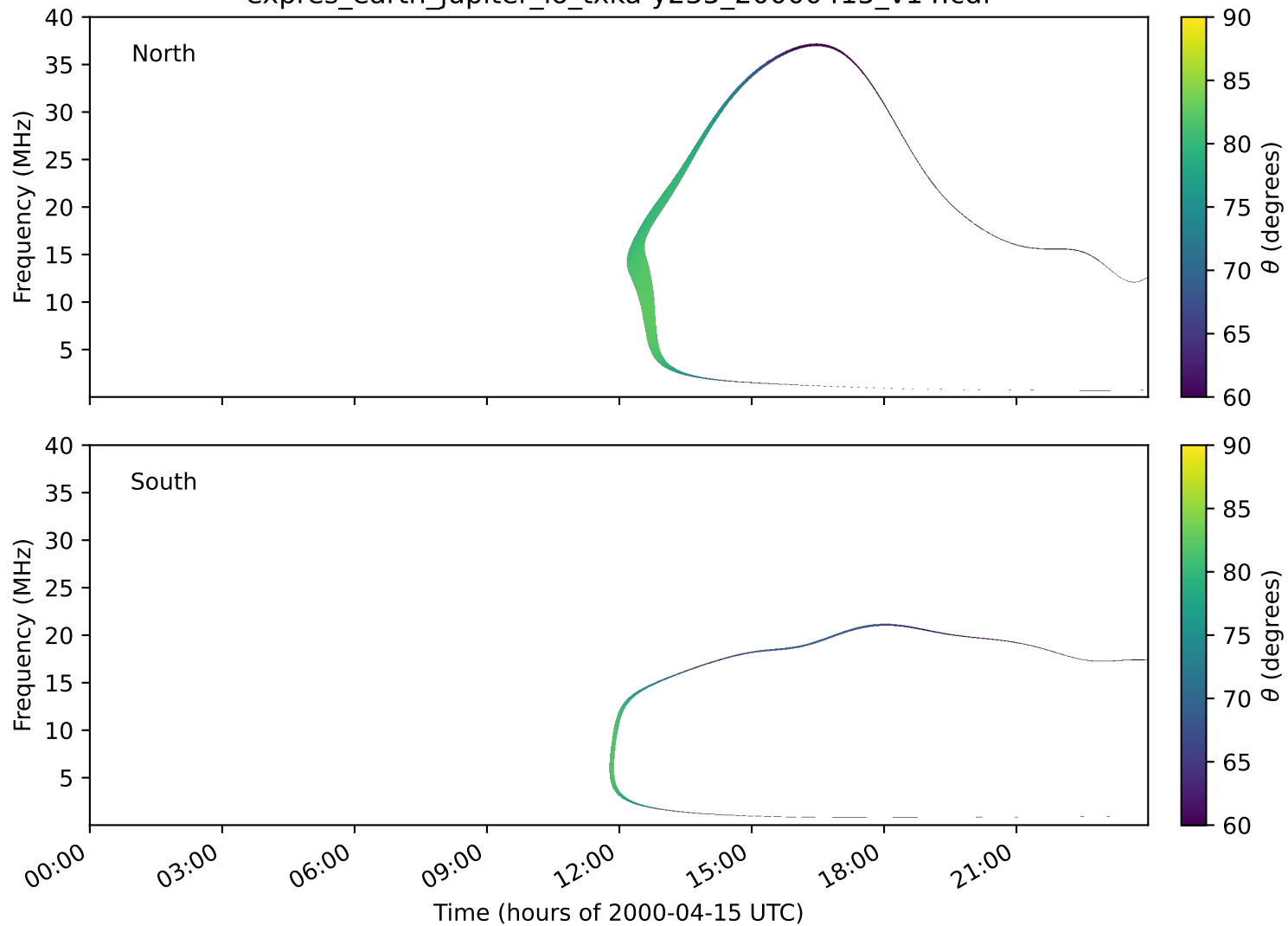
expres_earth_jupiter_io_txka-y235_20000415_v14.cdf
