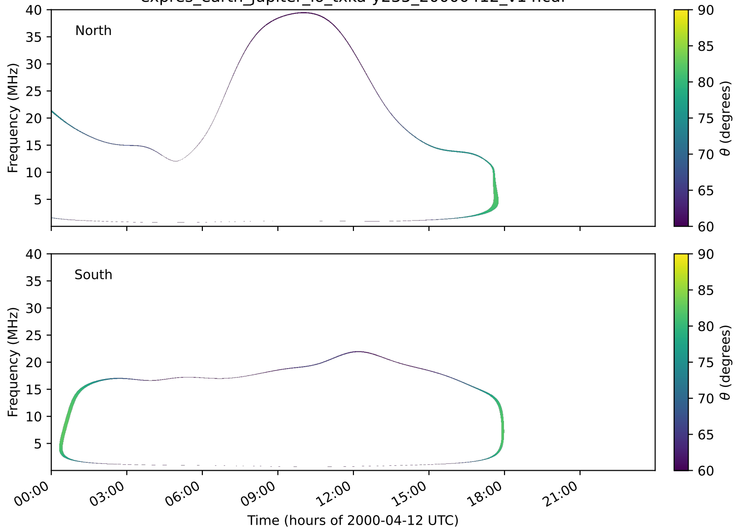
expres_earth_jupiter_io_txka-y235_20000412_v14.cdf
