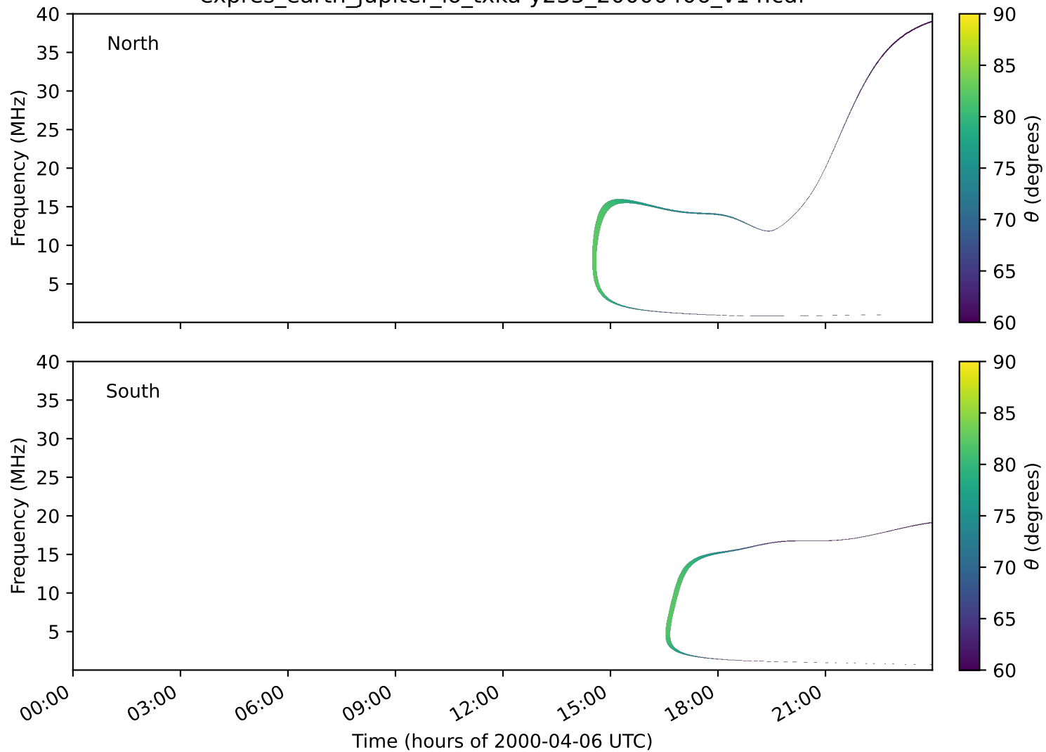
expres_earth_jupiter_io_txka-y235_20000406_v14.cdf
