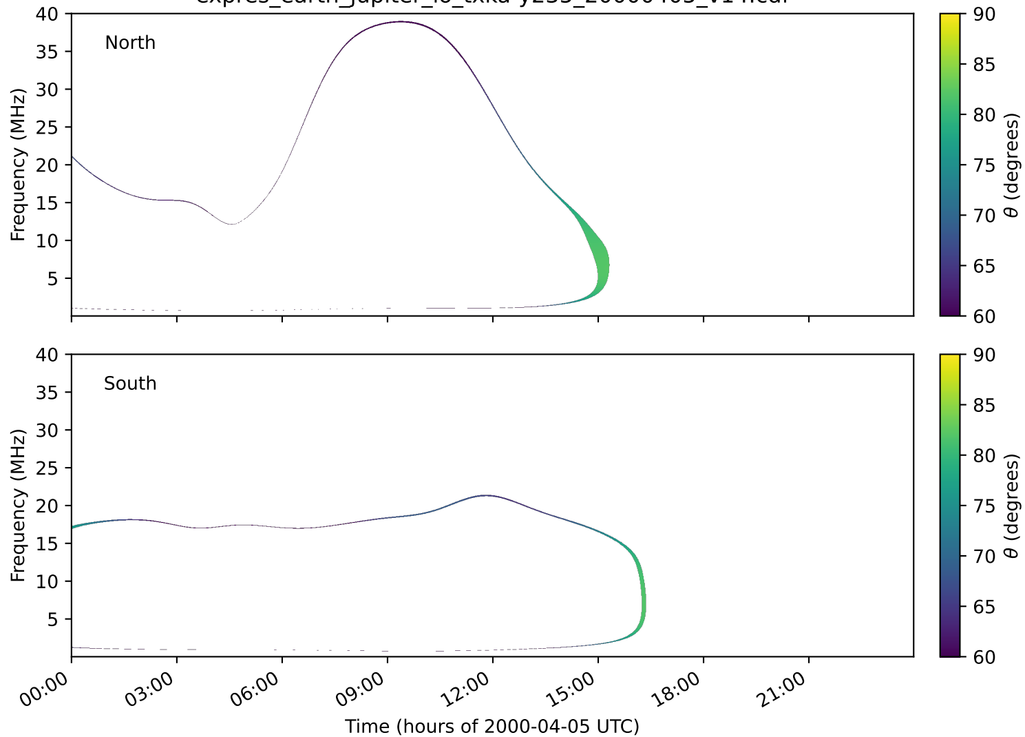
expres_earth_jupiter_io_txka-y235_20000405_v14.cdf
