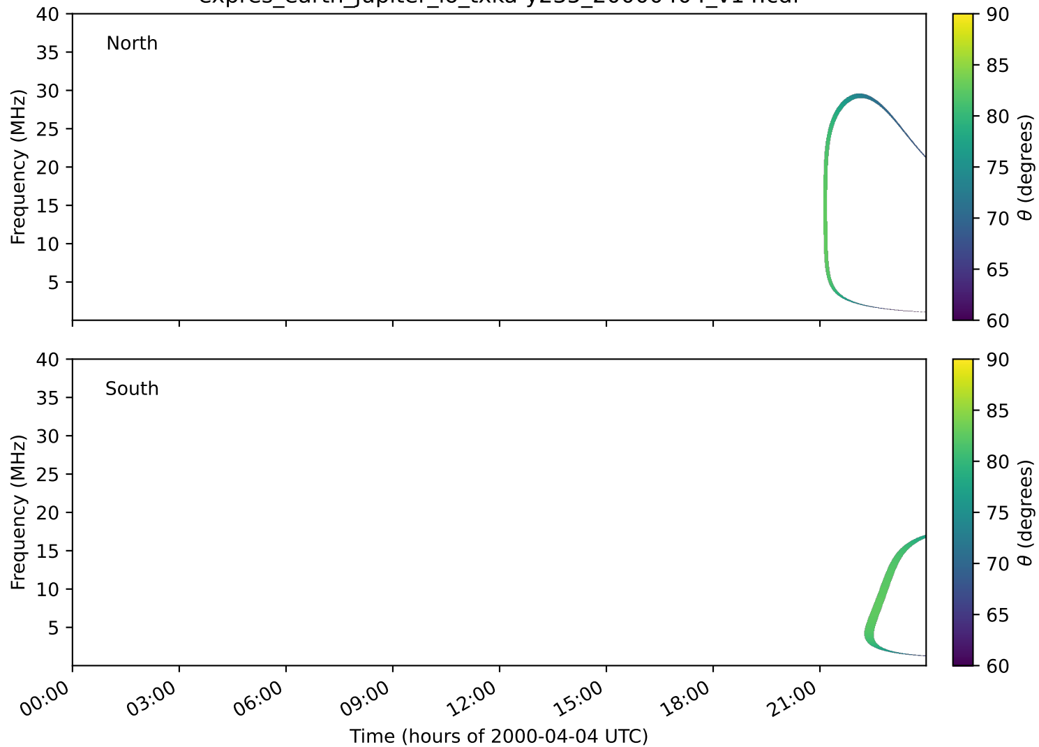
expres_earth_jupiter_io_txka-y235_20000404_v14.cdf
