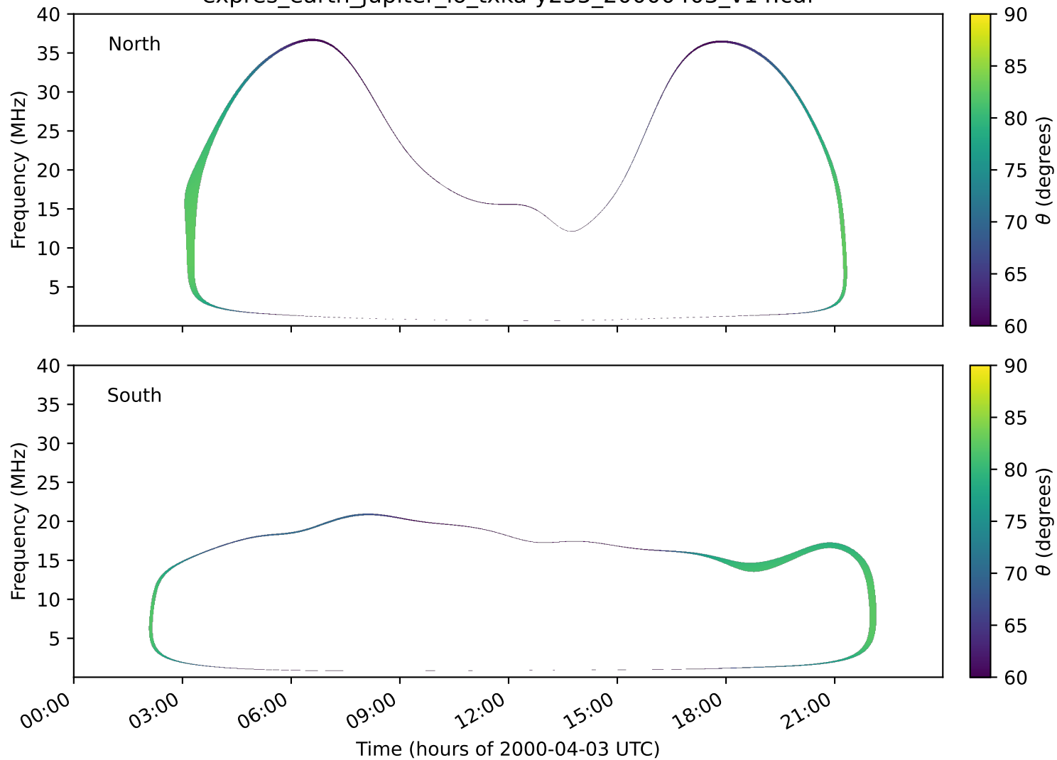
expres_earth_jupiter_io_txka-y235_20000403_v14.cdf
