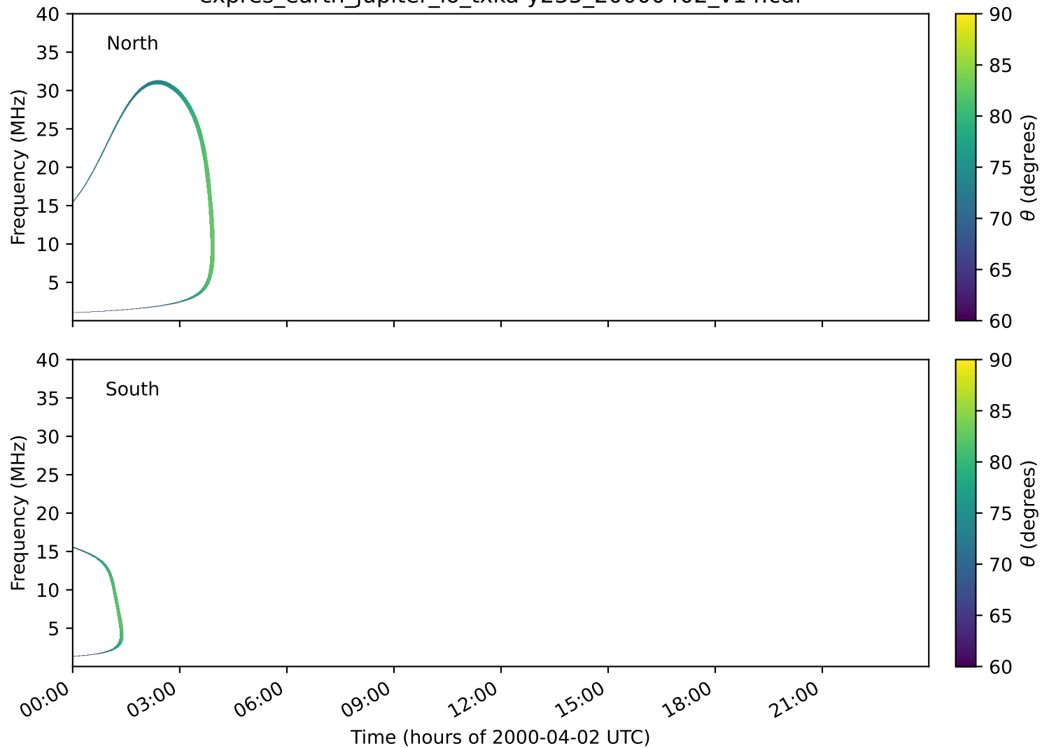
expres_earth_jupiter_io_txka-y235_20000402_v14.cdf
