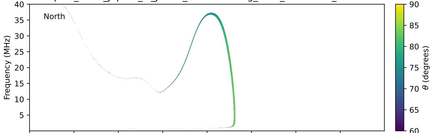
expres_earth_jupiter_io_jrm33_lossc-wid1deg_3kev_20000414_v11.cdf
