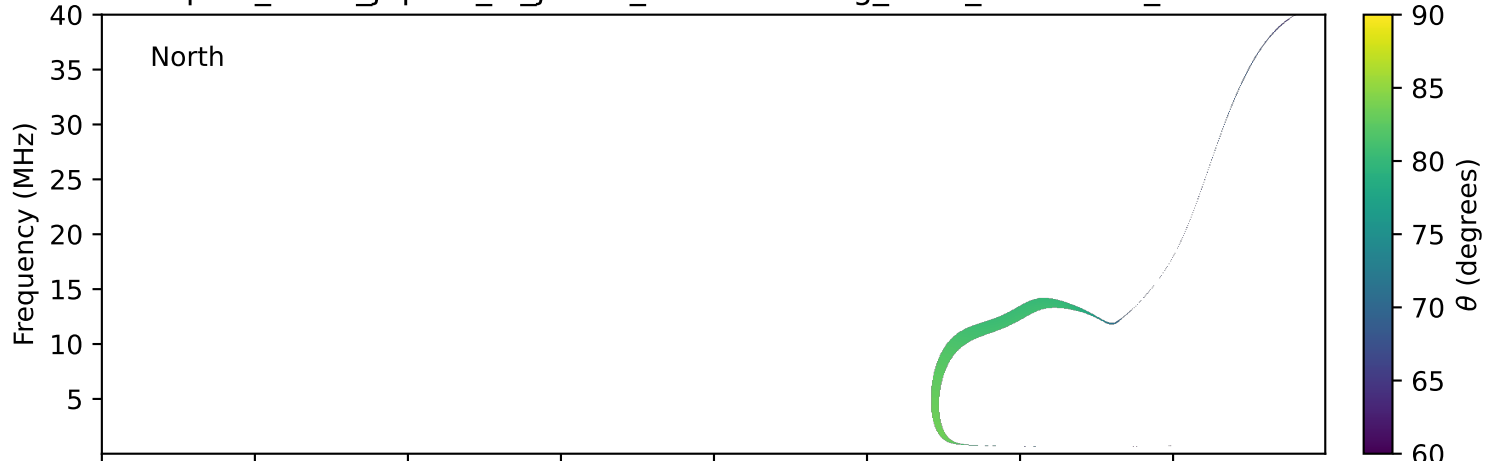
expres_earth_jupiter_io_jrm33_lossc-wid1deg_3kev_20000413_v11.cdf
