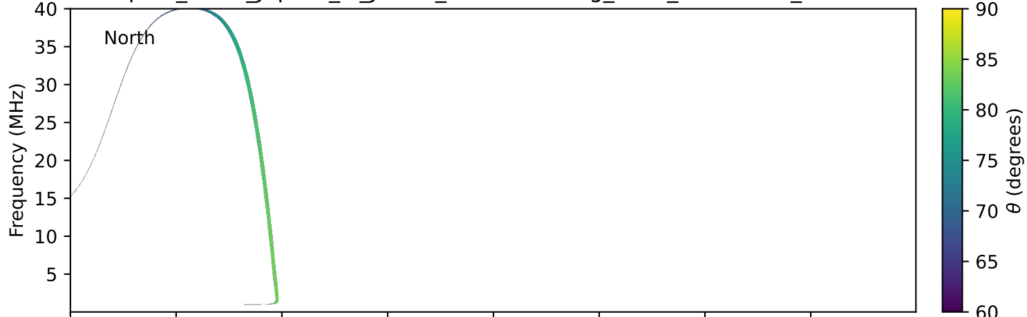
expres_earth_jupiter_io_jrm33_lossc-wid1deg_3kev_20000409_v11.cdf
