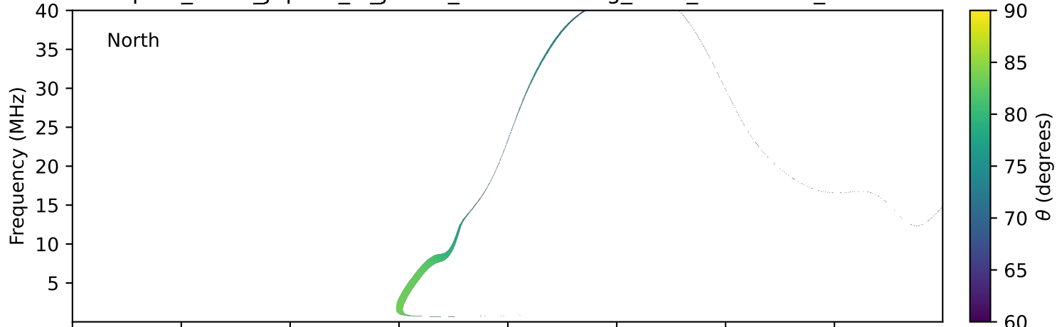
expres_earth_jupiter_io_jrm33_lossc-wid1deg_3kev_20000408_v11.cdf
