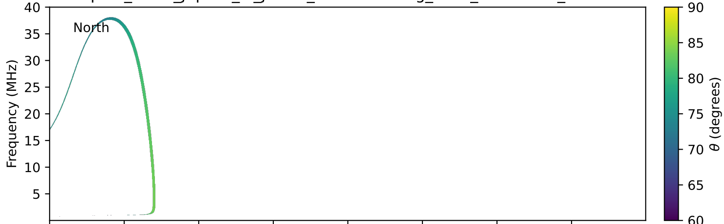
expres_earth_jupiter_io_jrm33_lossc-wid1deg_3kev_20000402_v11.cdf
