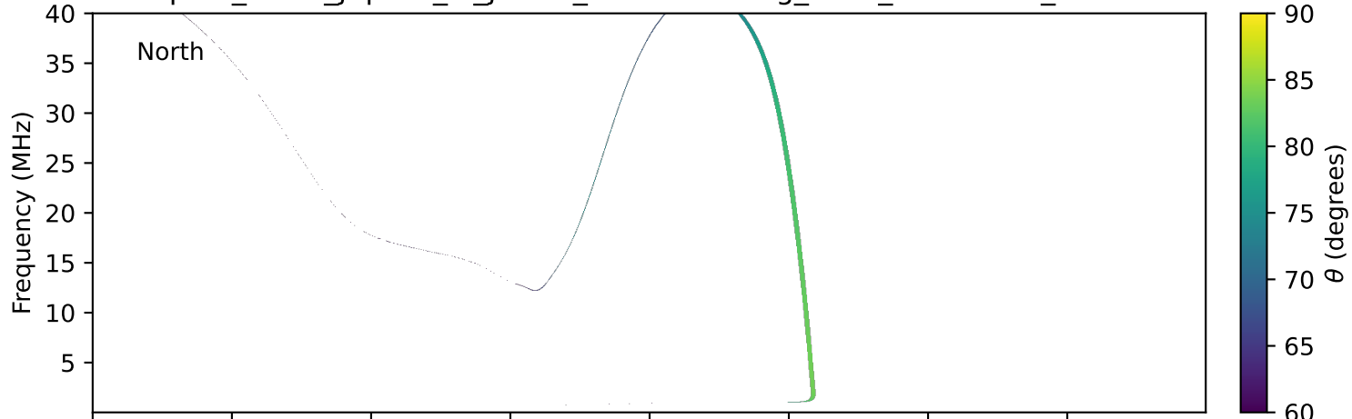
expres_earth_jupiter_io_jrm09_lossc-wid1deg_3kev_20000421_v11.cdf
