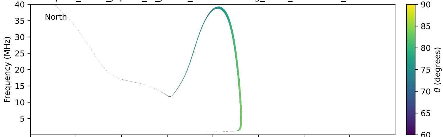
expres_earth_jupiter_io_jrm09_lossc-wid1deg_3kev_20000414_v11.cdf
