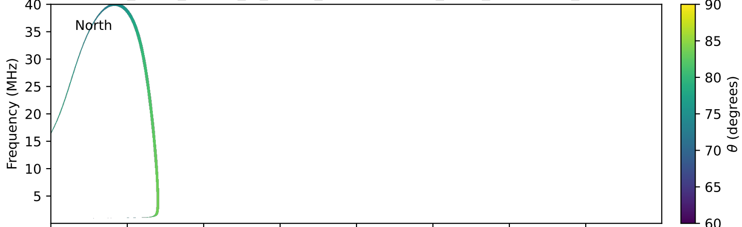
expres_earth_jupiter_io_jrm09_lossc-wid1deg_3kev_20000402_v11.cdf
