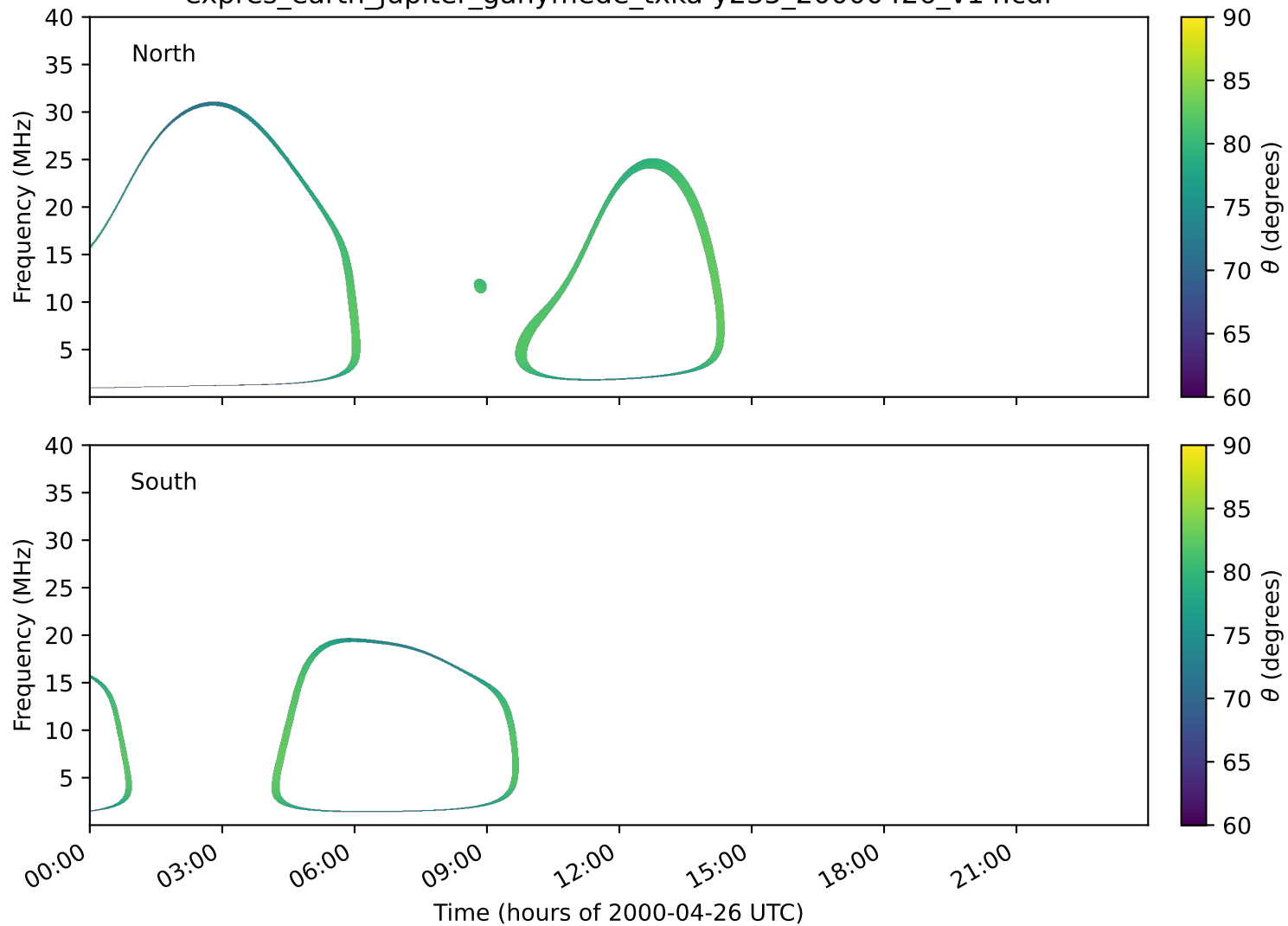
expres_earth_jupiter_ganymede_txka-y235_20000426_v14.cdf
