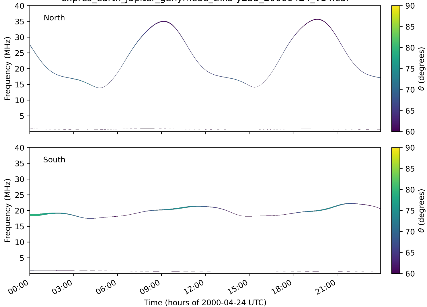
expres_earth_jupiter_ganymede_txka-y235_20000424_v14.cdf
