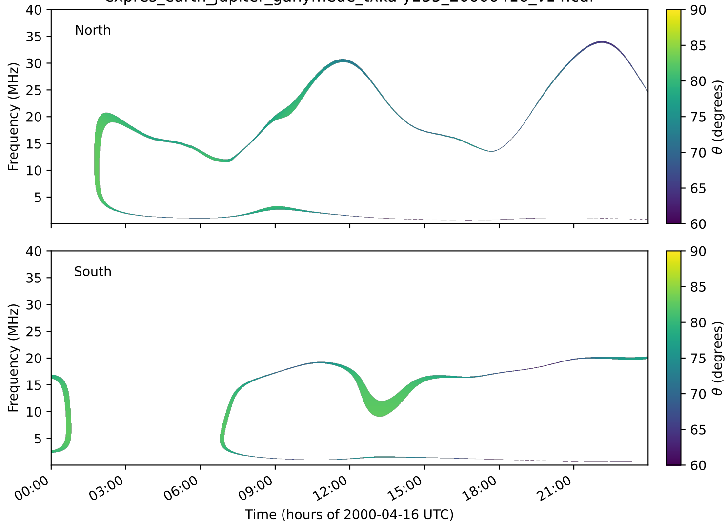
expres_earth_jupiter_ganymede_txka-y235_20000416_v14.cdf
