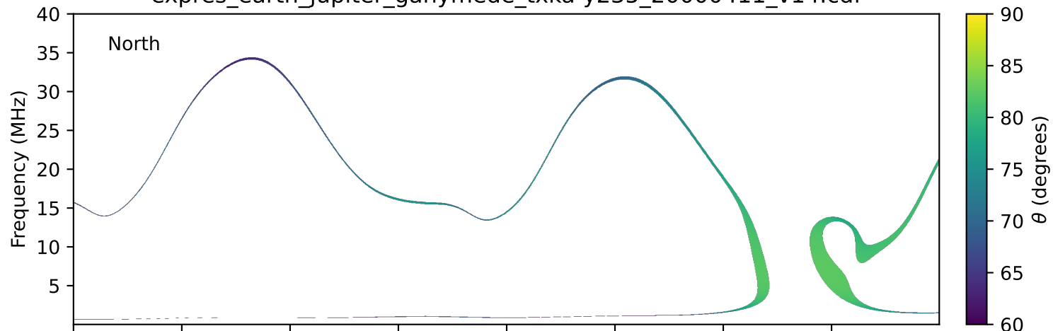
expres_earth_jupiter_ganymede_txka-y235_20000411_v14.cdf
