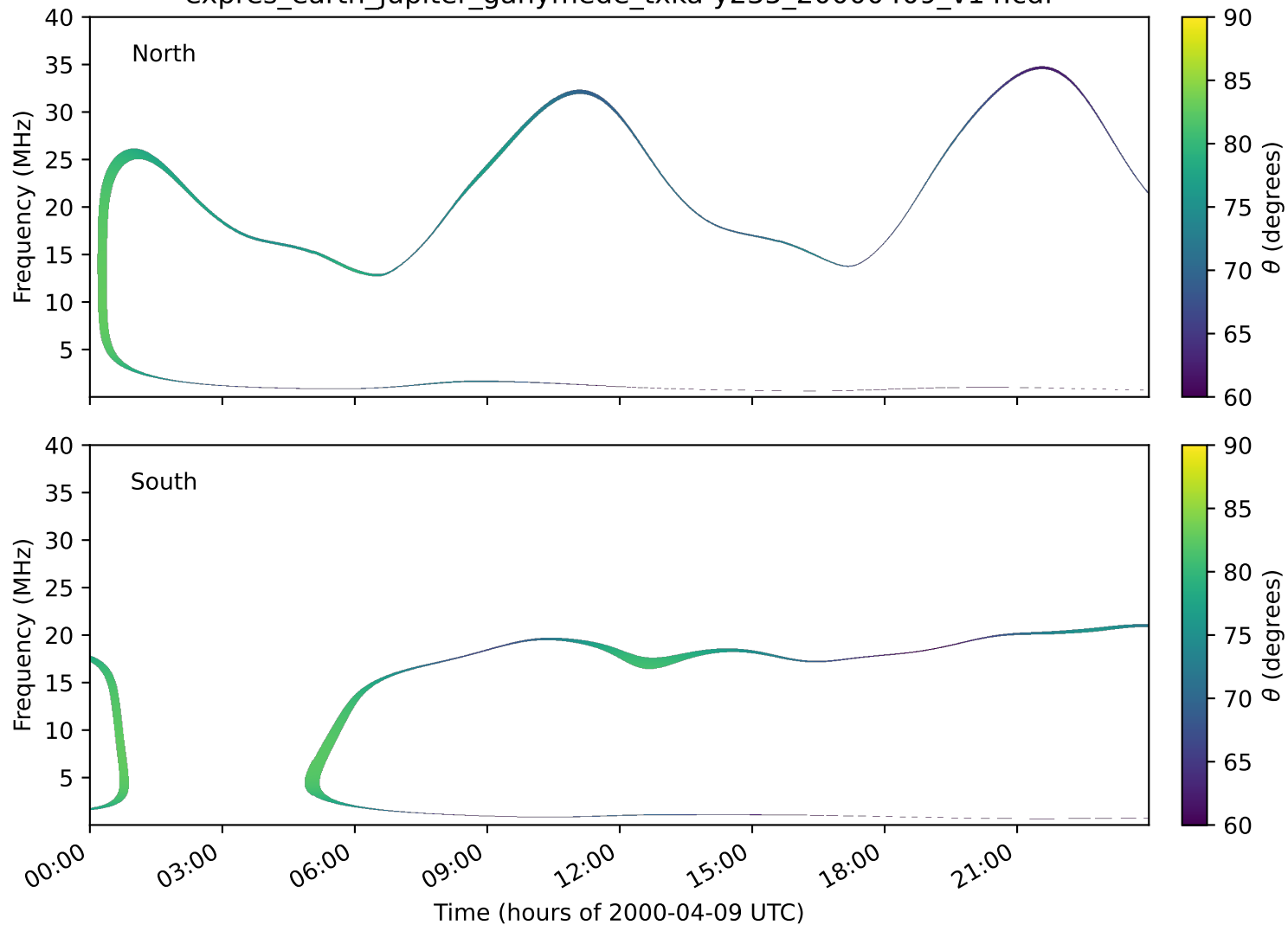
expres_earth_jupiter_ganymede_txka-y235_20000409_v14.cdf
