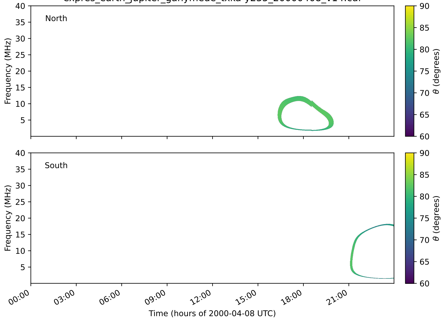
expres_earth_jupiter_ganymede_txka-y235_20000408_v14.cdf
