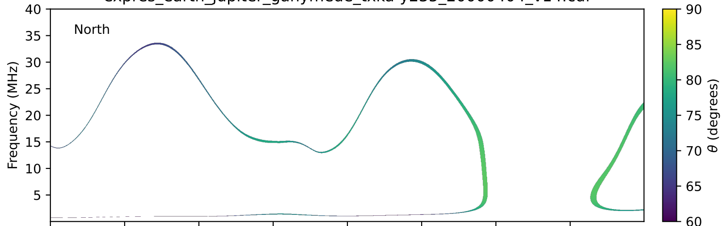
expres_earth_jupiter_ganymede_txka-y235_20000404_v14.cdf
