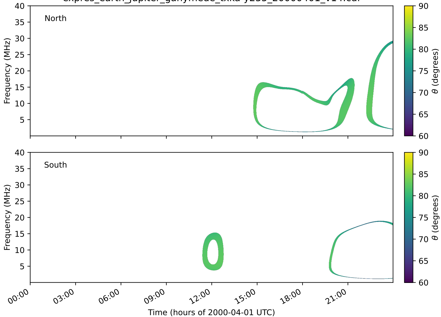
expres_earth_jupiter_ganymede_txka-y235_20000401_v14.cdf
