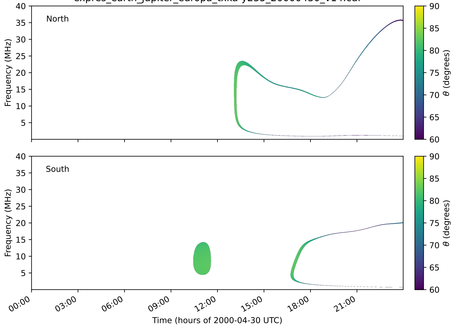
expres_earth_jupiter_europa_txka-y235_20000430_v14.cdf
