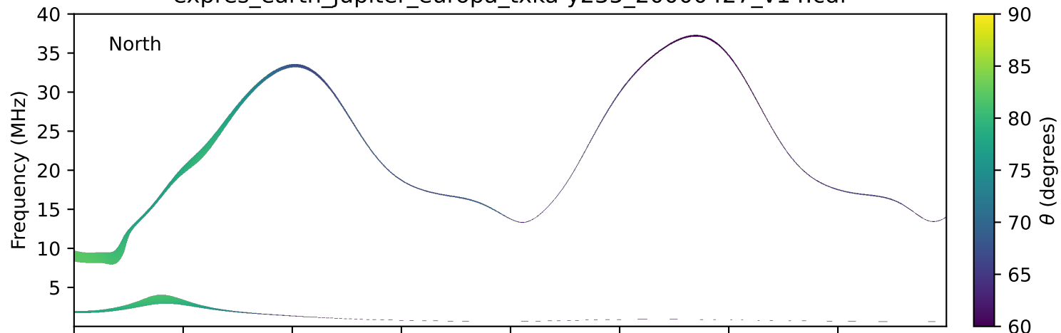
expres_earth_jupiter_europa_txka-y235_20000427_v14.cdf
