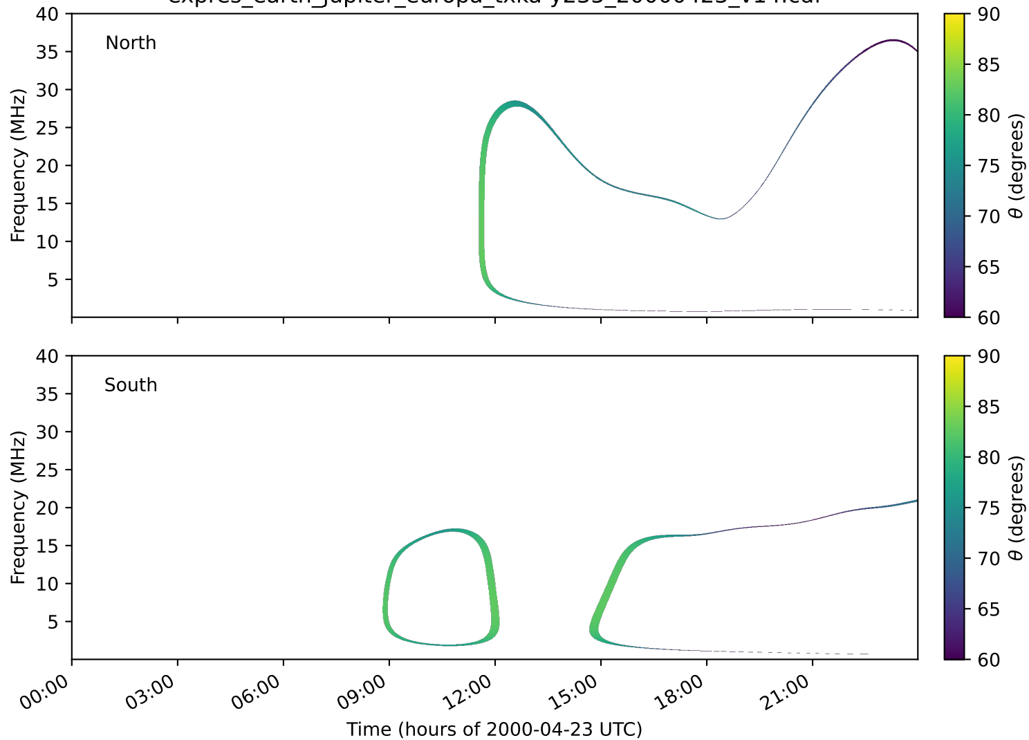
expres_earth_jupiter_europa_txka-y235_20000423_v14.cdf
