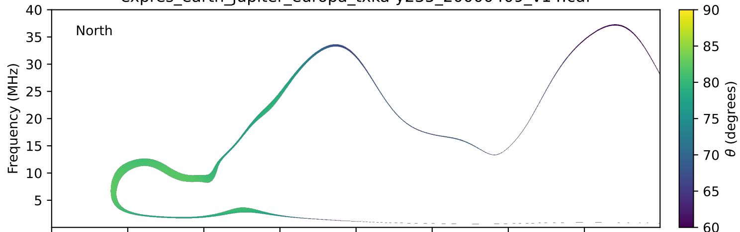
expres_earth_jupiter_europa_txka-y235_20000409_v14.cdf
