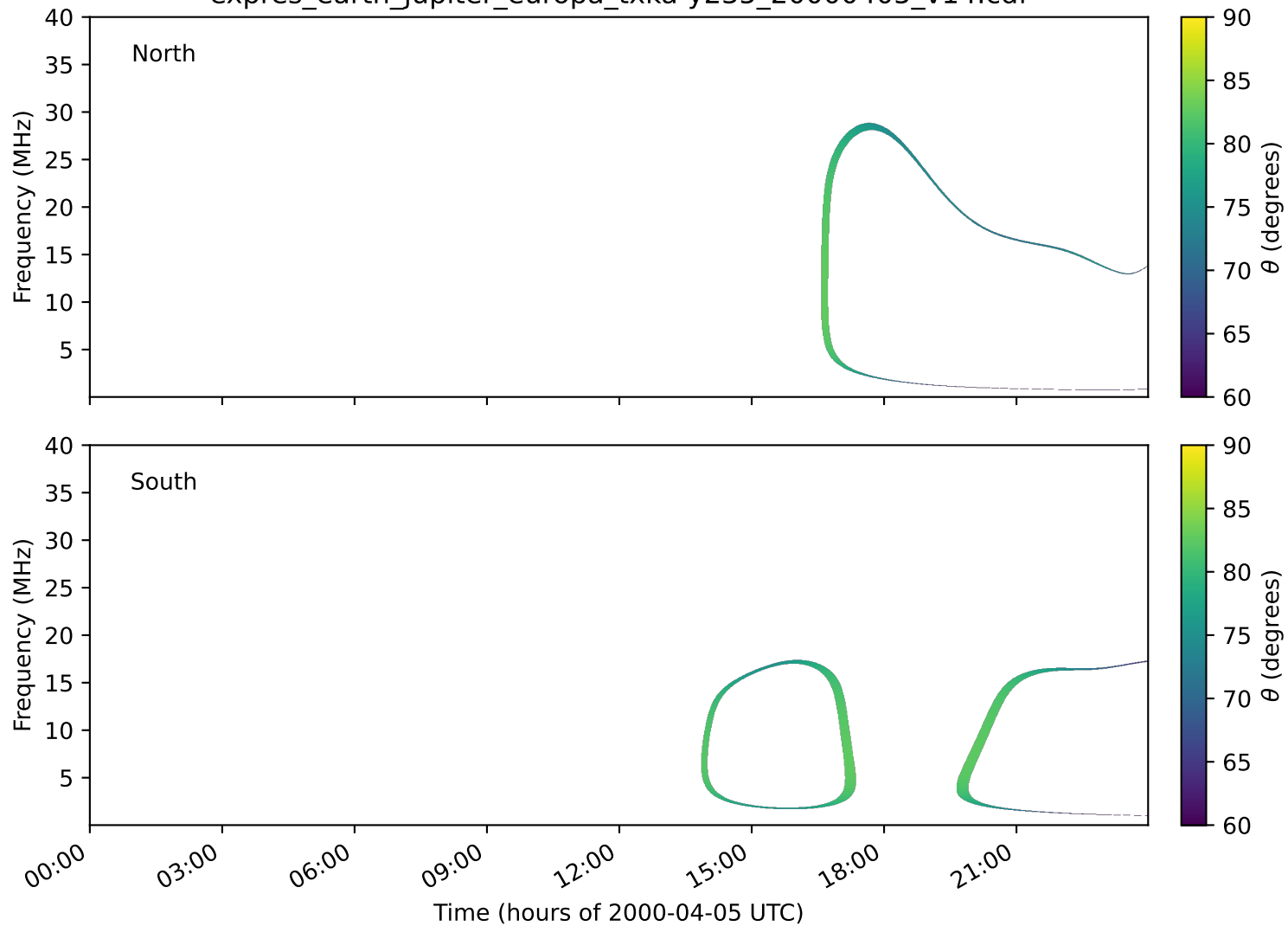
expres_earth_jupiter_europa_txka-y235_20000405_v14.cdf
