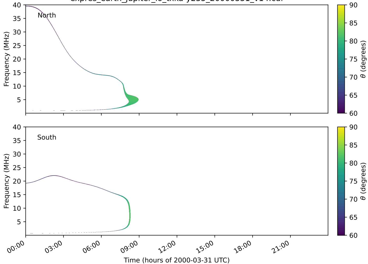
expres_earth_jupiter_io_txka-y235_20000331_v14.cdf
