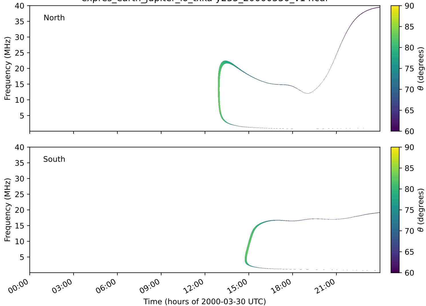
expres_earth_jupiter_io_txka-y235_20000330_v14.cdf
