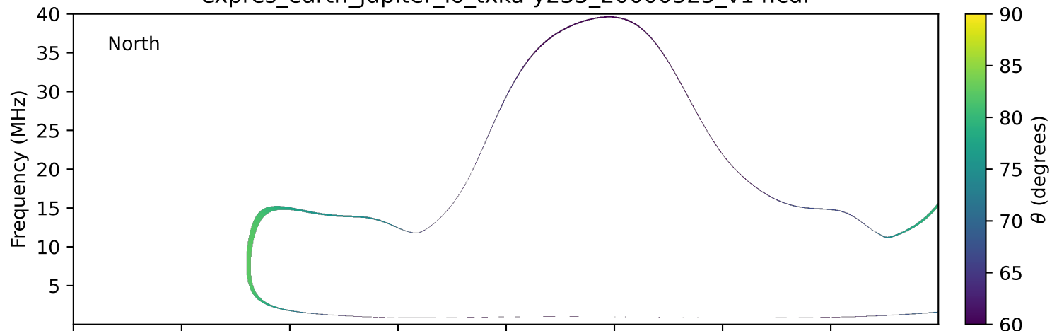
expres_earth_jupiter_io_txka-y235_20000325_v14.cdf
