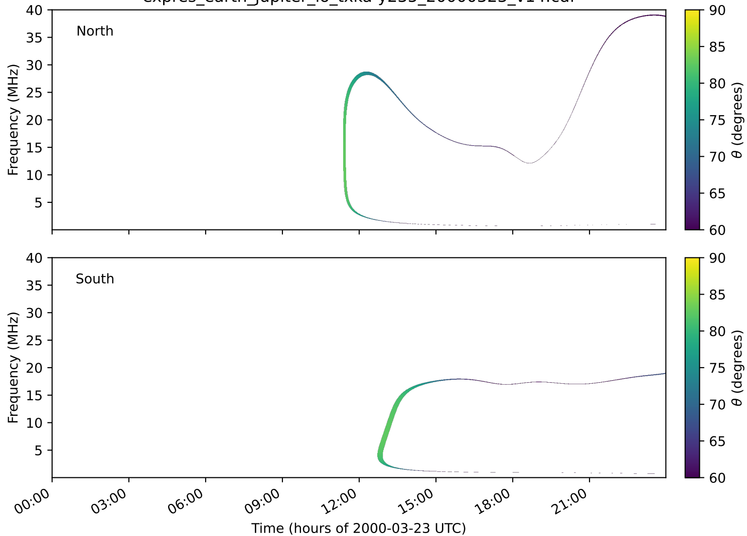
expres_earth_jupiter_io_txka-y235_20000323_v14.cdf
