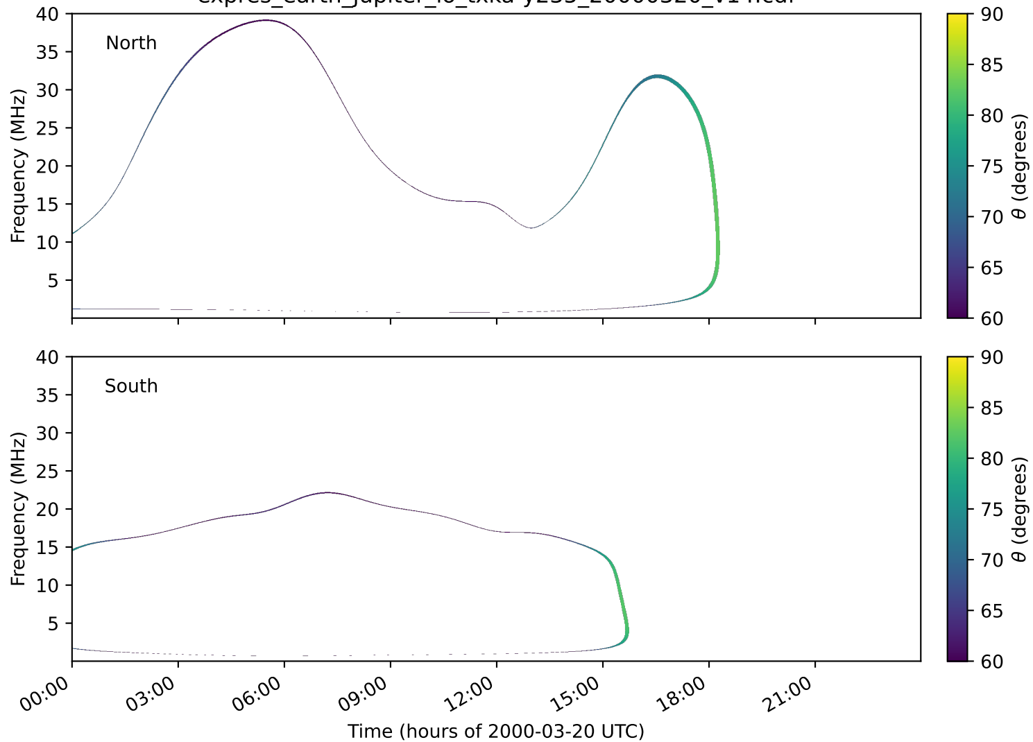
expres_earth_jupiter_io_txka-y235_20000320_v14.cdf
