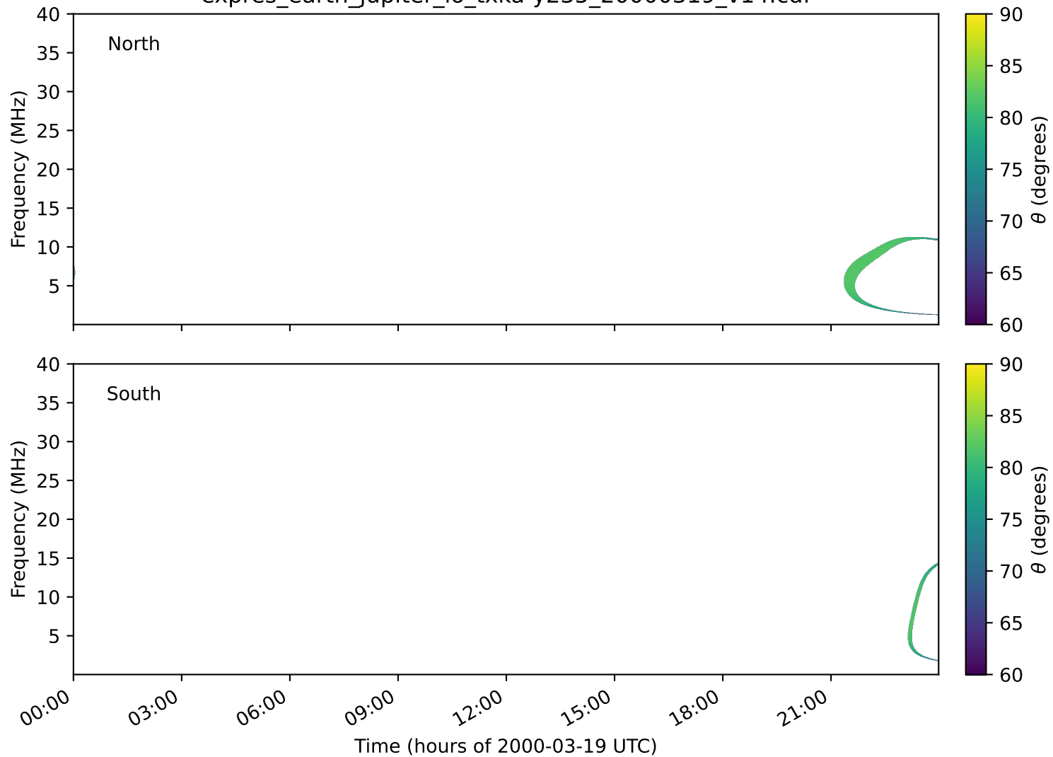
expres_earth_jupiter_io_txka-y235_20000319_v14.cdf
