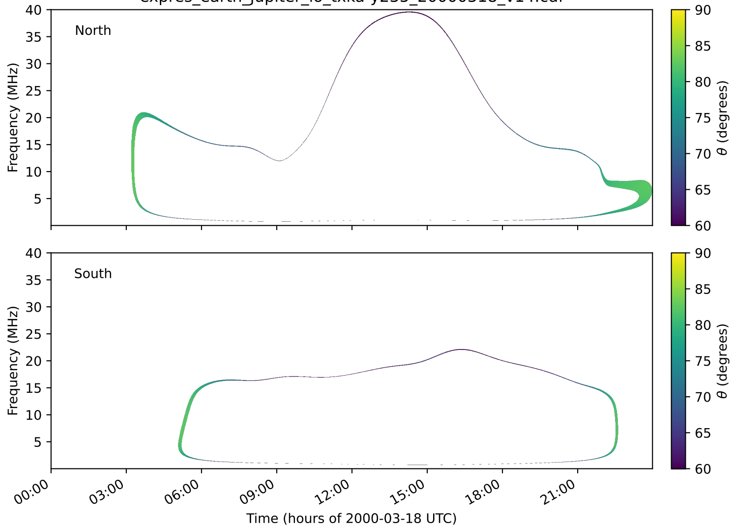
expres_earth_jupiter_io_txka-y235_20000318_v14.cdf
