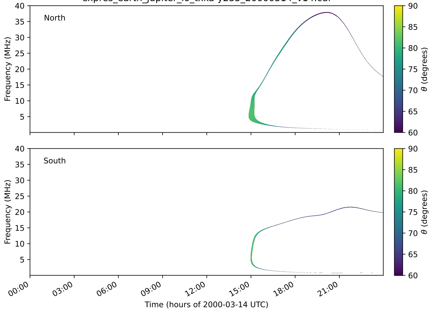
expres_earth_jupiter_io_txka-y235_20000314_v14.cdf
